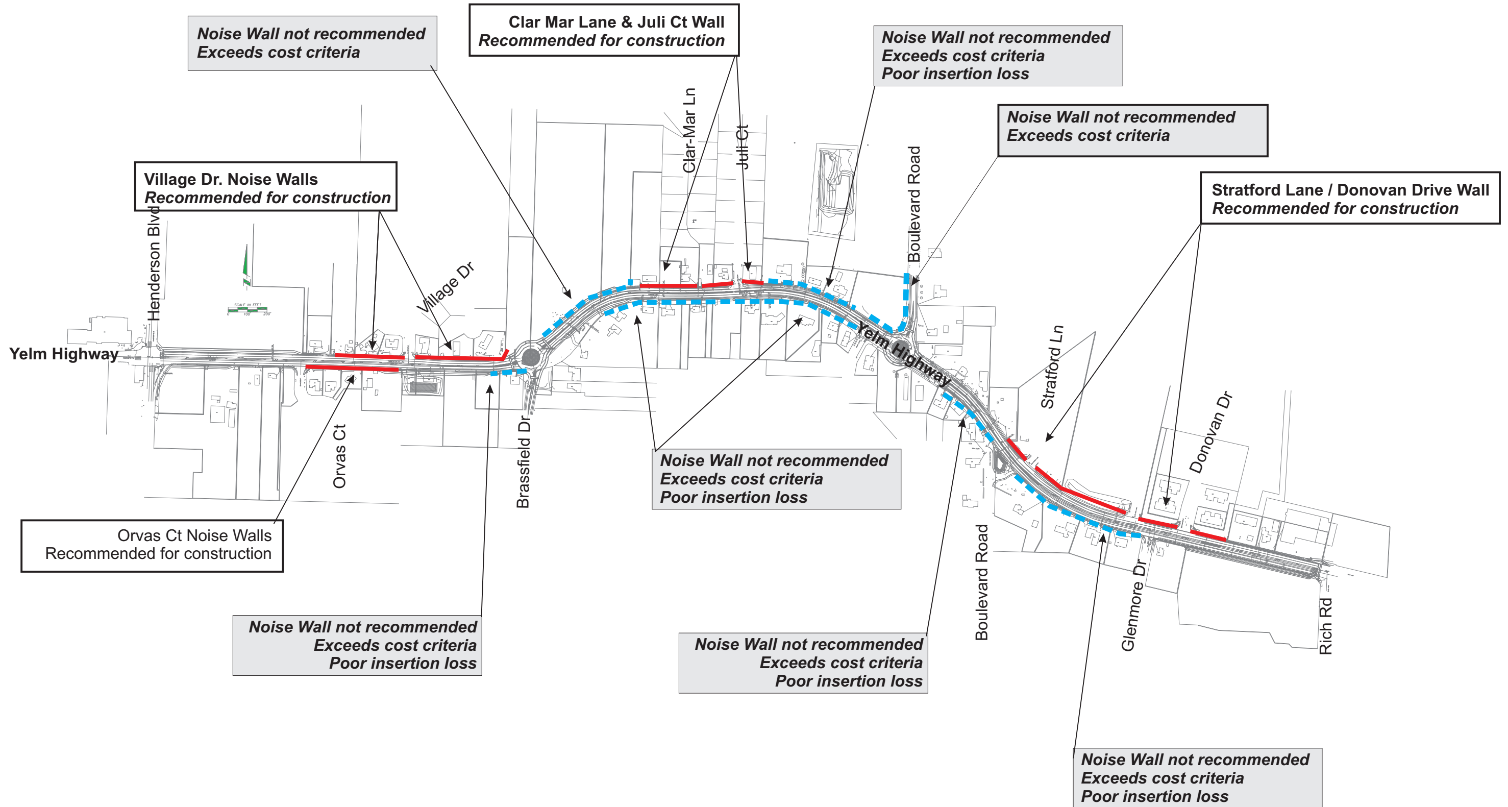
Figure 6 Noise Barriers Considered Under Revised Analysis Yelm Highway Improvement Project
