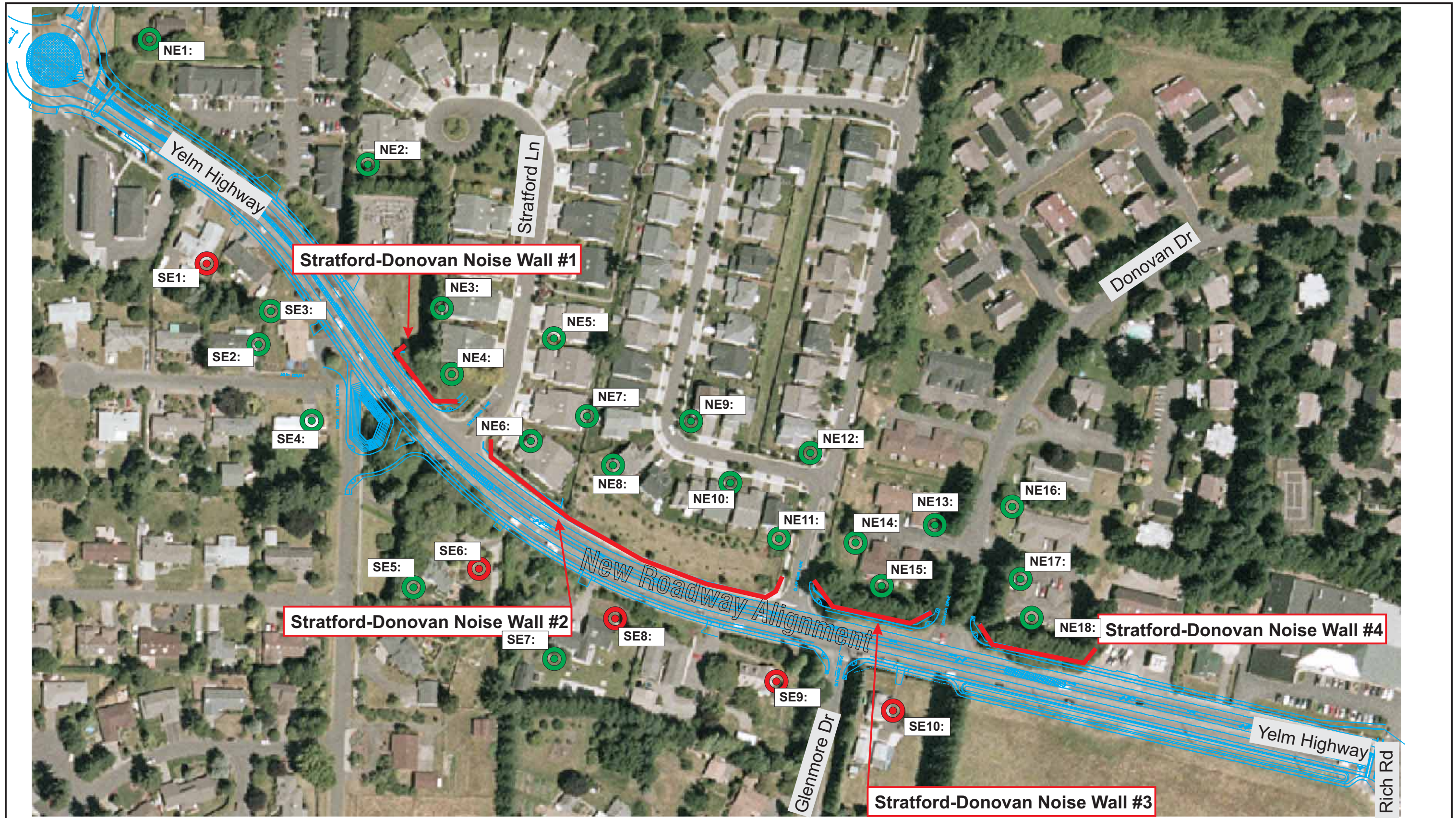
Figure 7C (figure 3 of 3) Future Build Noise Levels and Residual Noise Impacts Projected with recommended noise mitigation measures Yelm Highway Improvement Project
