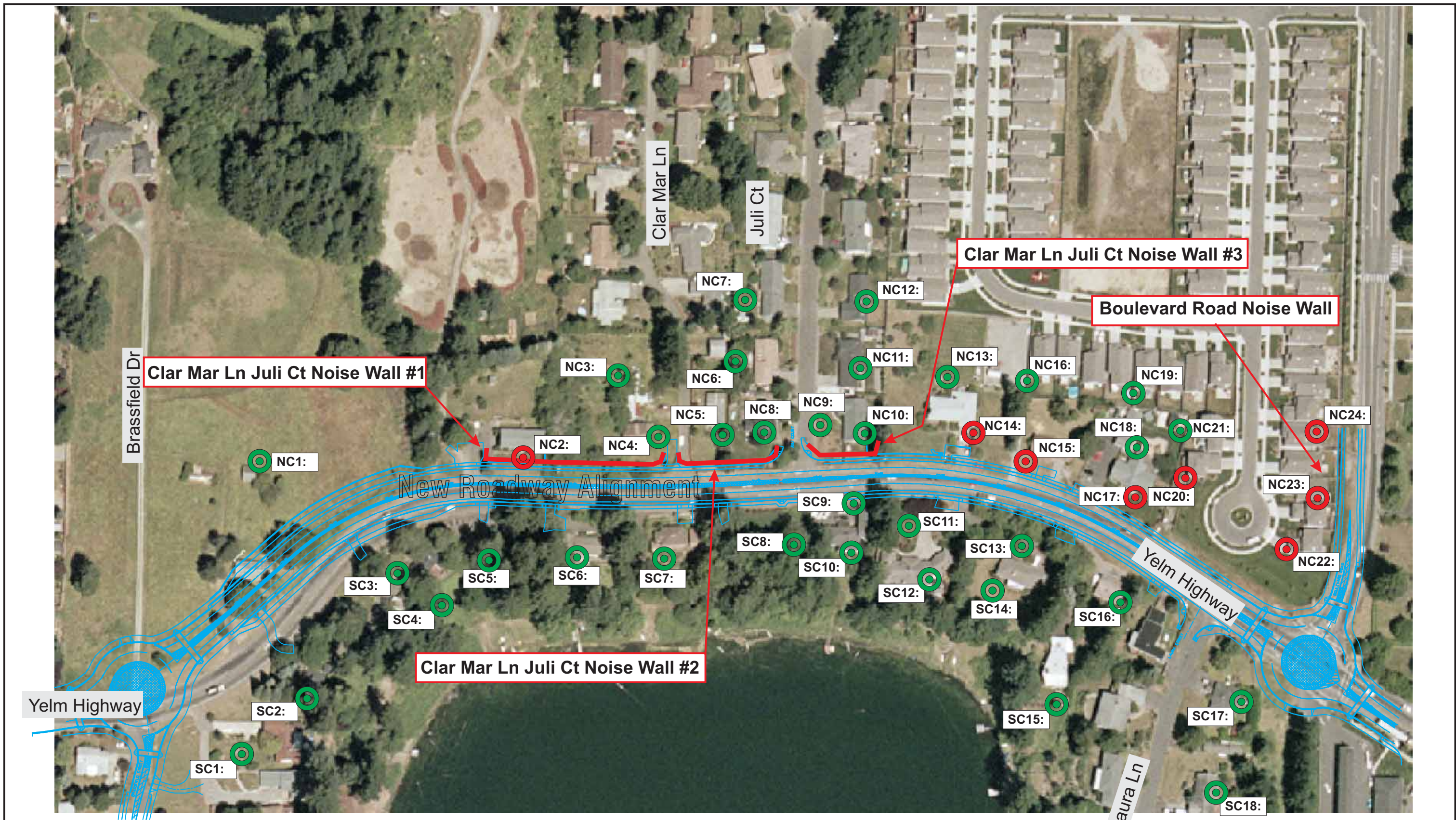
Figure 7B (figure 2 of 3) Future Build Noise Levels and Residual Noise Impacts Projected with recommended noise mitigation measures Yelm Highway Improvement Project
