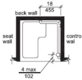
Transfer Shower Grab Bars
