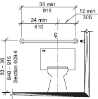
Grab Bar for Water Closets (toilets)
