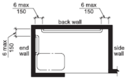
Alternate Roll-in Type Shower
