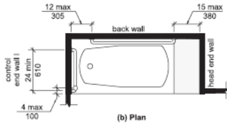
(b) Plan
