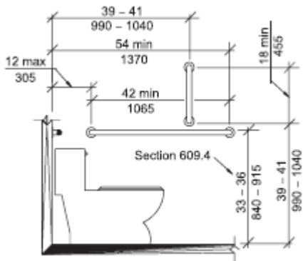
Grab Bar for Water Closets (toilets)
